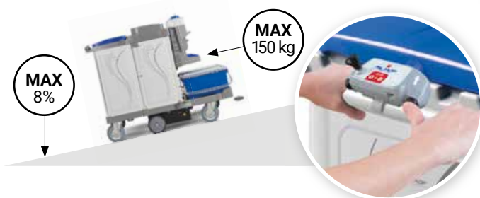
Control console with switch-on key
